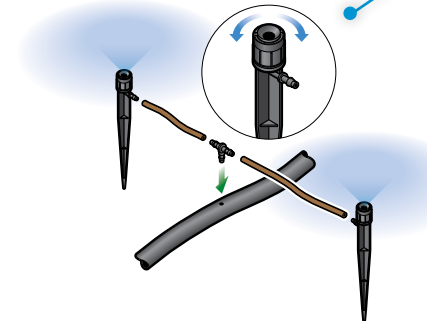
micro sprayers 101
